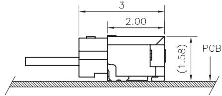
MATED CONDITION
