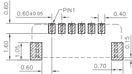
RECOMMEND PCB LAYOUT GENERAL TOLERANCE ±0.05
